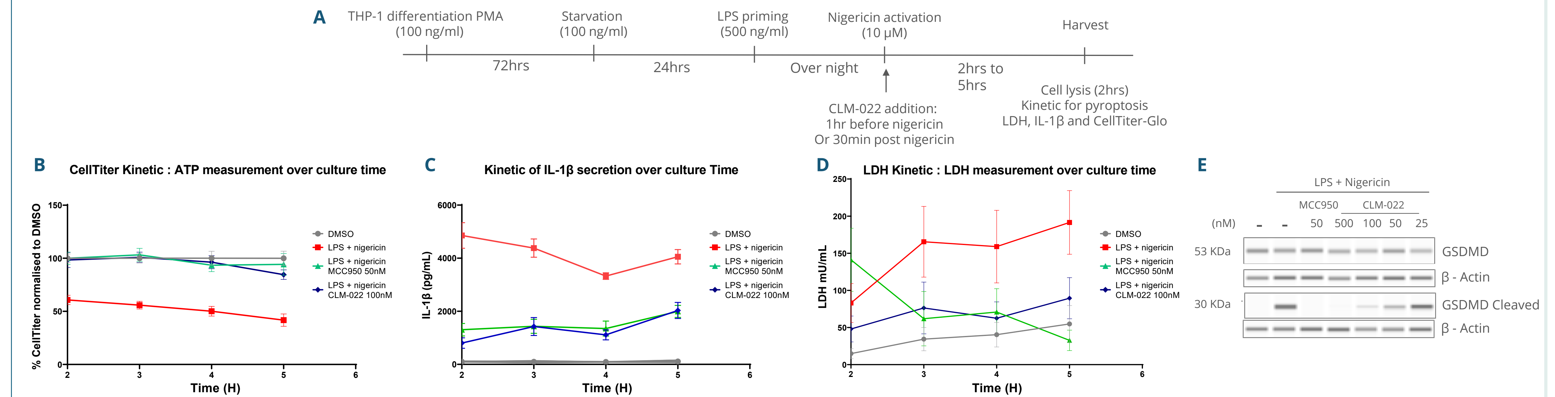
Figure 4: CLM-022 inhibits pyroptosis
